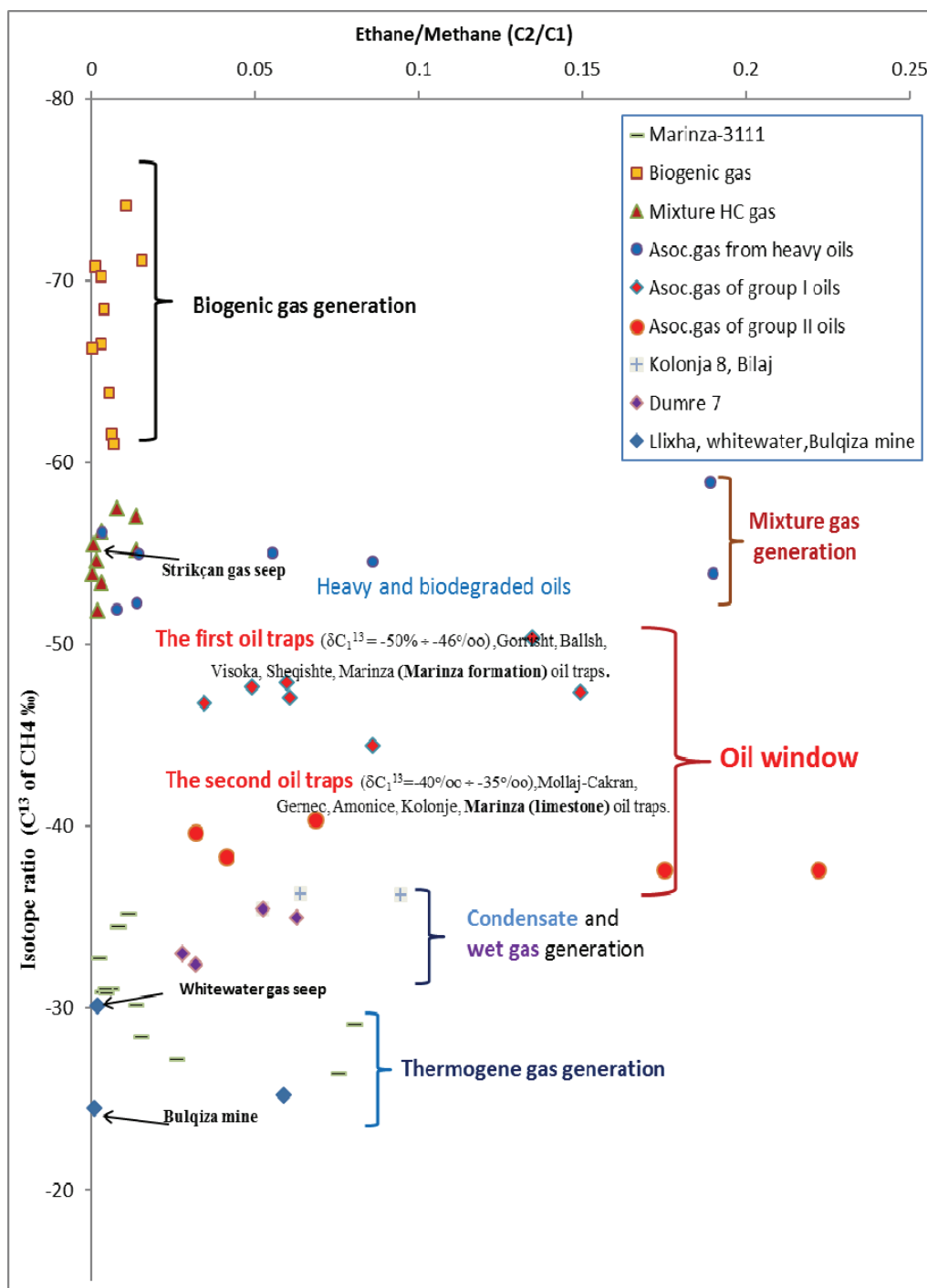
Figure 5. The position of hydrocarbon gasses from the Marinza-3111 well on the geochemical model of petroleum generation (based on SHKURTAJ et al., 2002, modification by Prifti and Seitaj).
